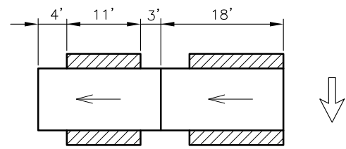
TANDEM STALLS (WITH APPROVAL OF COMMUNITY DEVELOPMENT DIRECTOR AND AS ALLOWED IN E-4 OF ENG. STANDARD #2020.)
